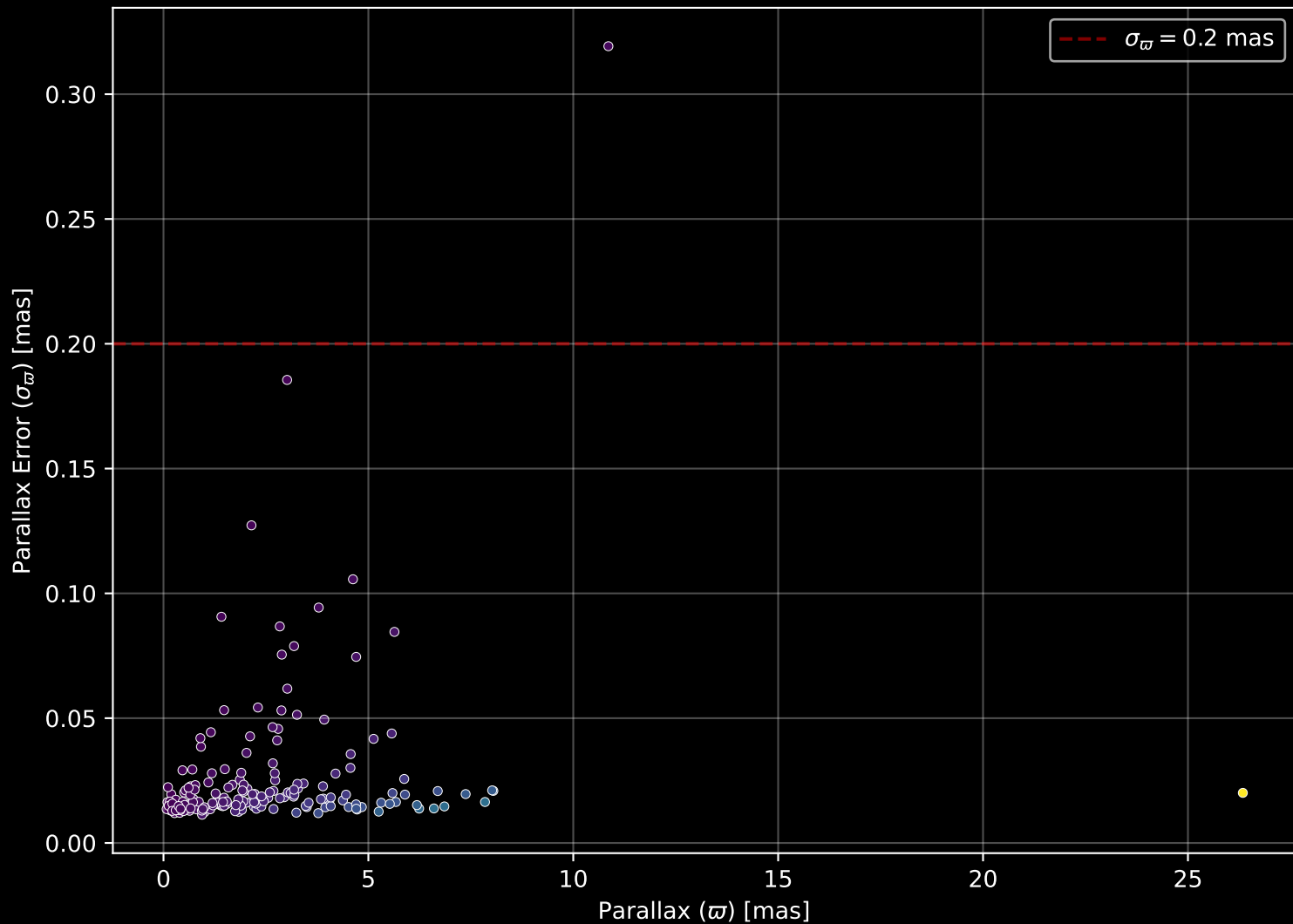
APOGEE DR17 Field: [175+26_MGA] Parallax Quality (n= 186)
