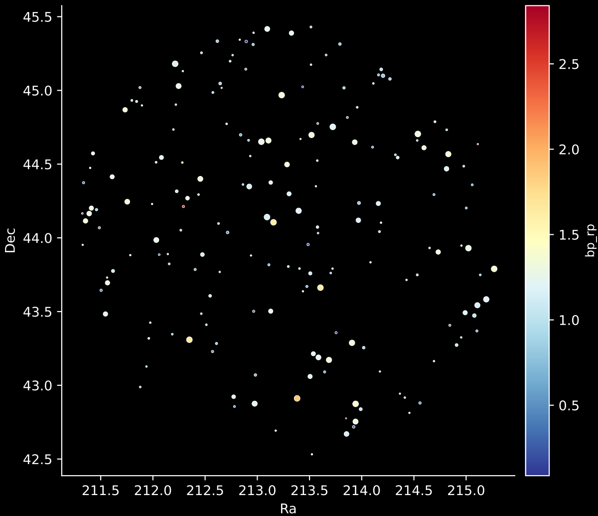
APOGEE DR17 Field: [175+26_MGA] Stars: 186
