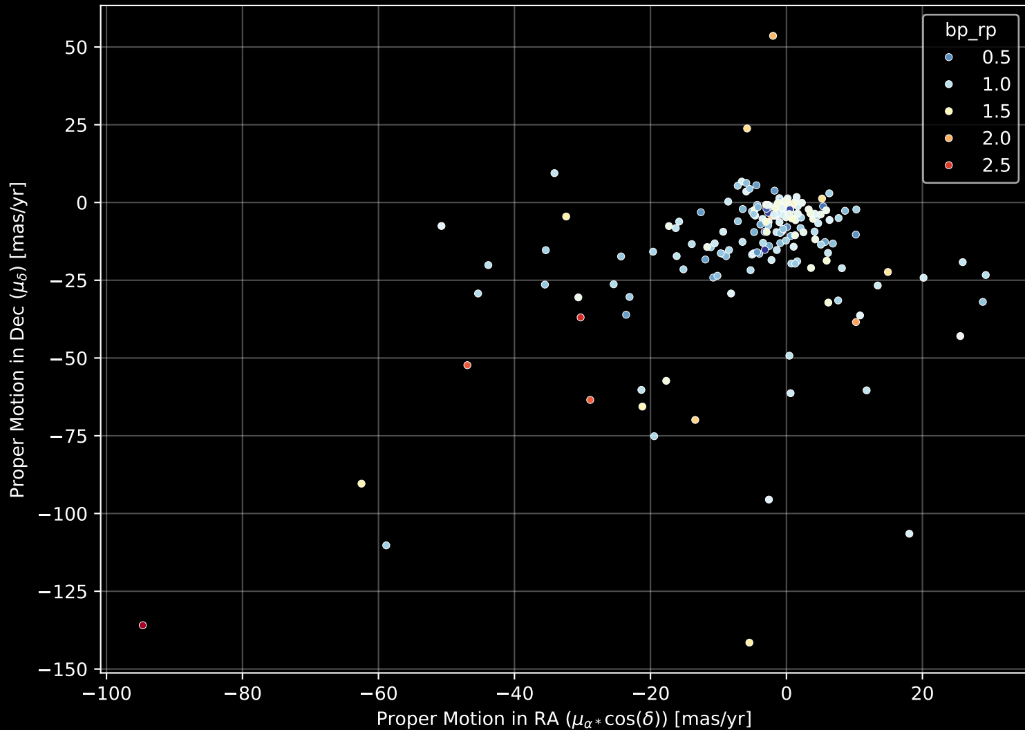
APOGEE DR17 Field: [175+26_MGA] Proper Motion Diagram (n= 186)
