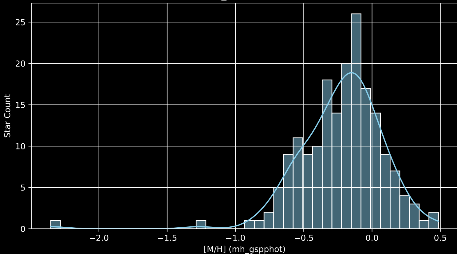
APOGEE DR17 Field: [175+26_MGA [M/H] (mh_gspphot) (n= 185)
