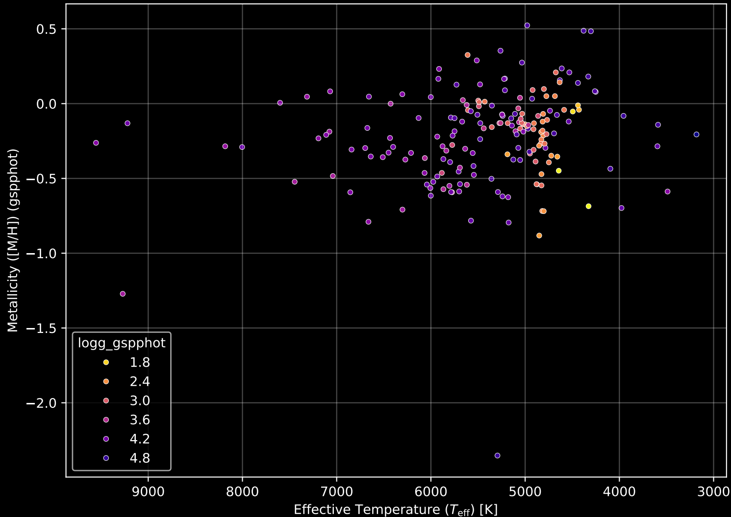
APOGEE DR17 Field: [175+26_MGA] Stellar Population Parameters (n= 186)
