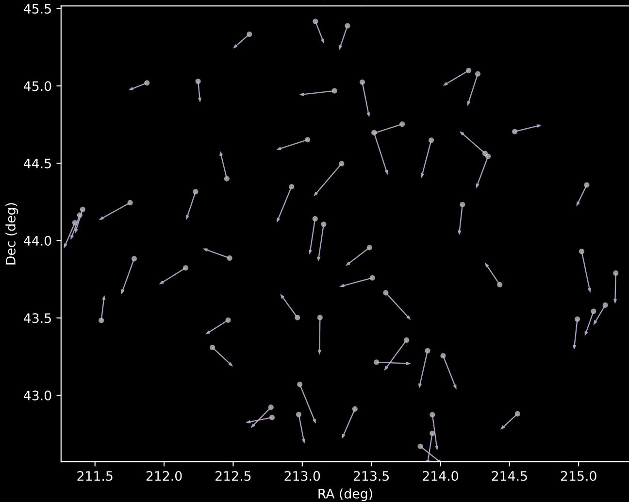
APOGEE DR17 Cluster 9 Proper Motion Vectors (n=58)
