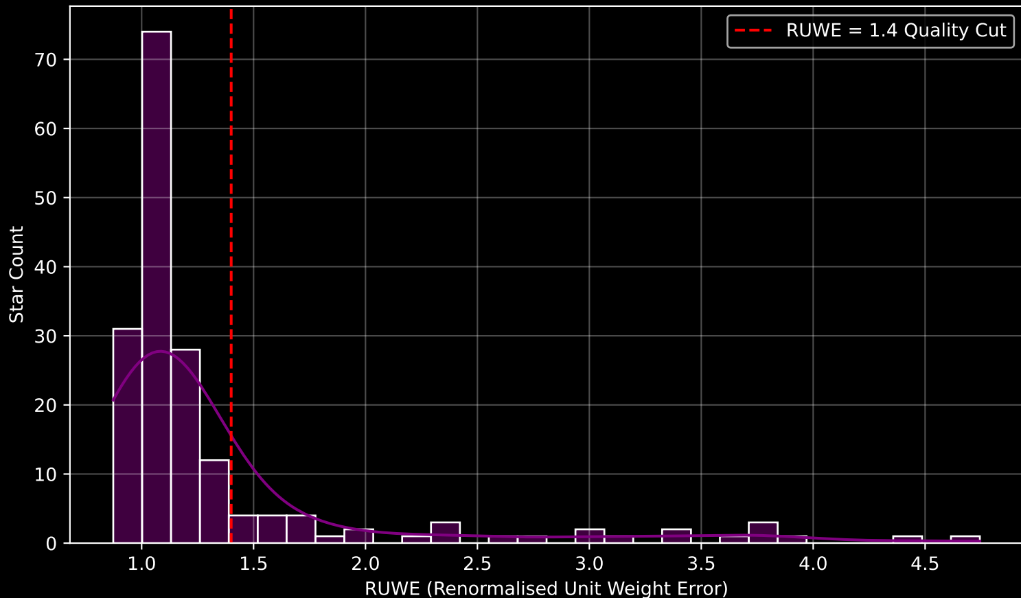
GAPOGEE DR17 Field [175+26_MGA] RUWE Distribution (n= 178)
