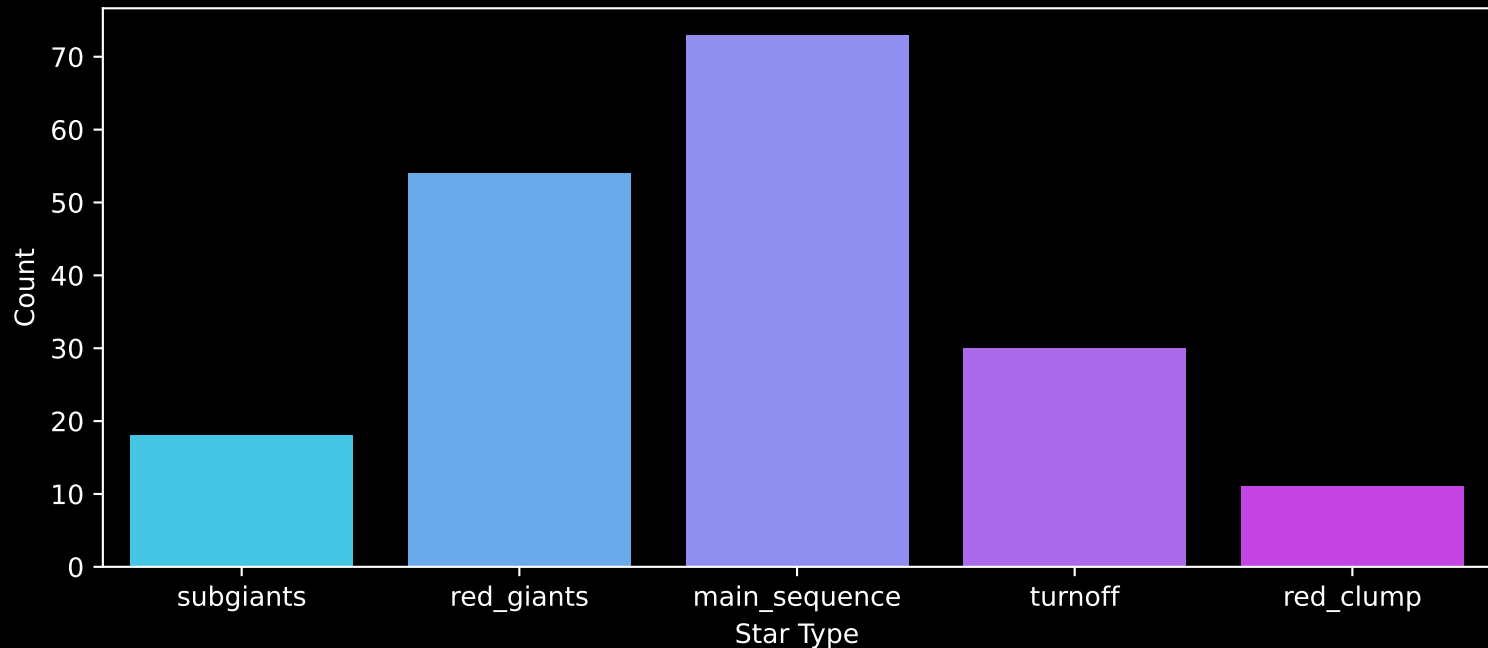
APOGEE DR17 Field: [175+26_MGA] Count plot of Star Type
